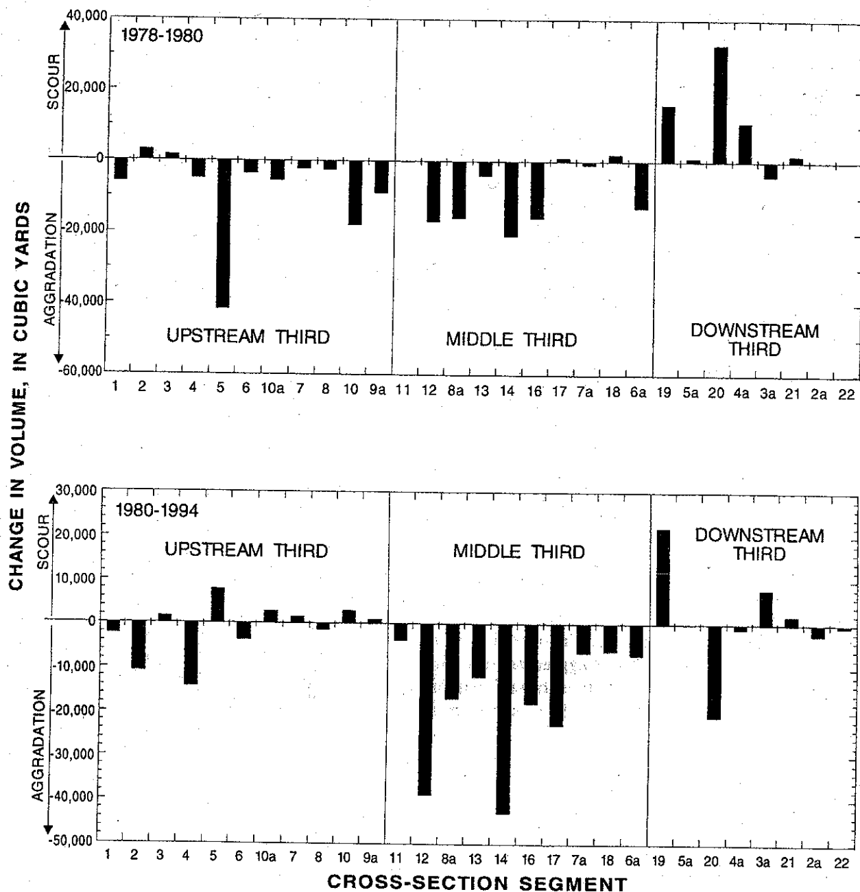
Figure 10. Changes in channel volume of the 29 cross-section segments in the Six-Mile Pool reach of the Kankakee River in Illinois, 1980-94 and 1978-80.
